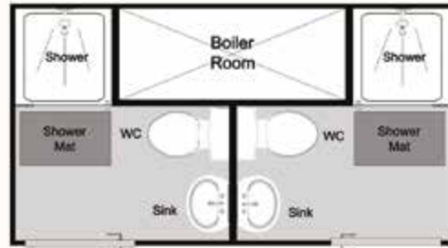
Double Shower & WC Pitch Pod
